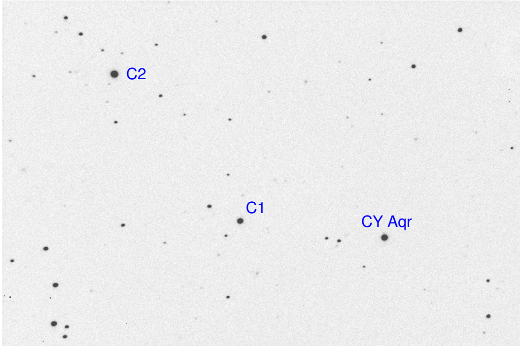
Figure 1: CY Aqr CCD field, from Sterken et al. (2011) . North is up and East is left, field of view is 18' \times 12' . CY Aqr and the comparison stars C_1 = \text{GSC } 00567-01826 and C_2 = \text{GSC } 00567-02036 are marked.
