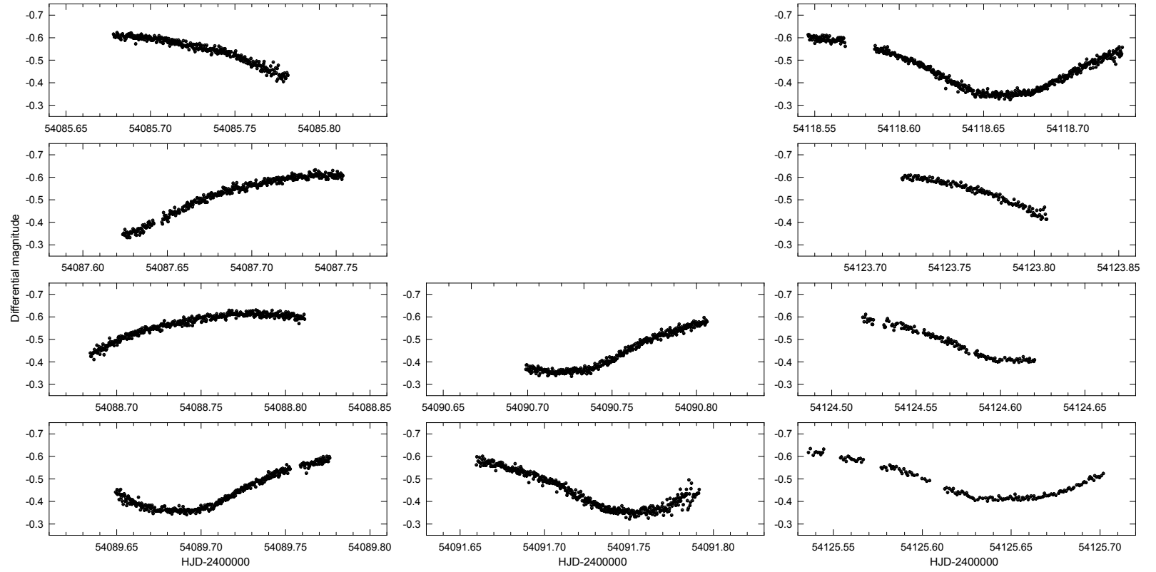
Figure 3: Overview of all OCA filterless light curves of GSC04778-00152: Dec 2006 (left and middle), January 2007 (right).
