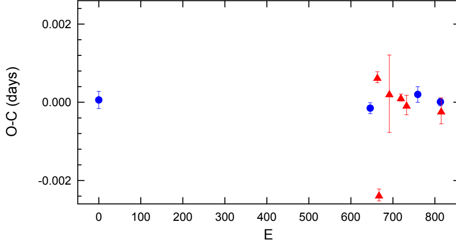
Figure 6: O - C diagram for GSC 04778–00152 constructed with ephemeris (1). \bullet : data from Tuvikene et al. (2008), \blacktriangle : results from this paper.
