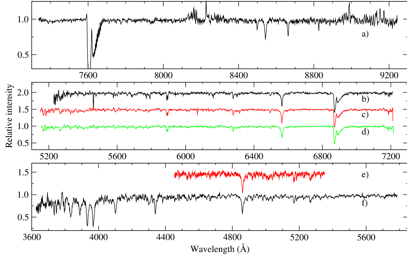
Figure 5: Low and medium resolution normalised spectra of GSC 04778-00152, see Table 5 for details.
