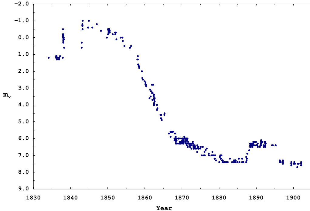
Figure 4: Visual light curve covering the period 1830–1910, to be compared with Fig. 1. The Great Eruption extended from 1837 to \sim 1856 . Note the constant rates of decline over the intervals 1845–56, 1858–68, and 1872–82, the plateau (or slight brightening) around 1870, and the Lesser Eruption of 1887–95.
