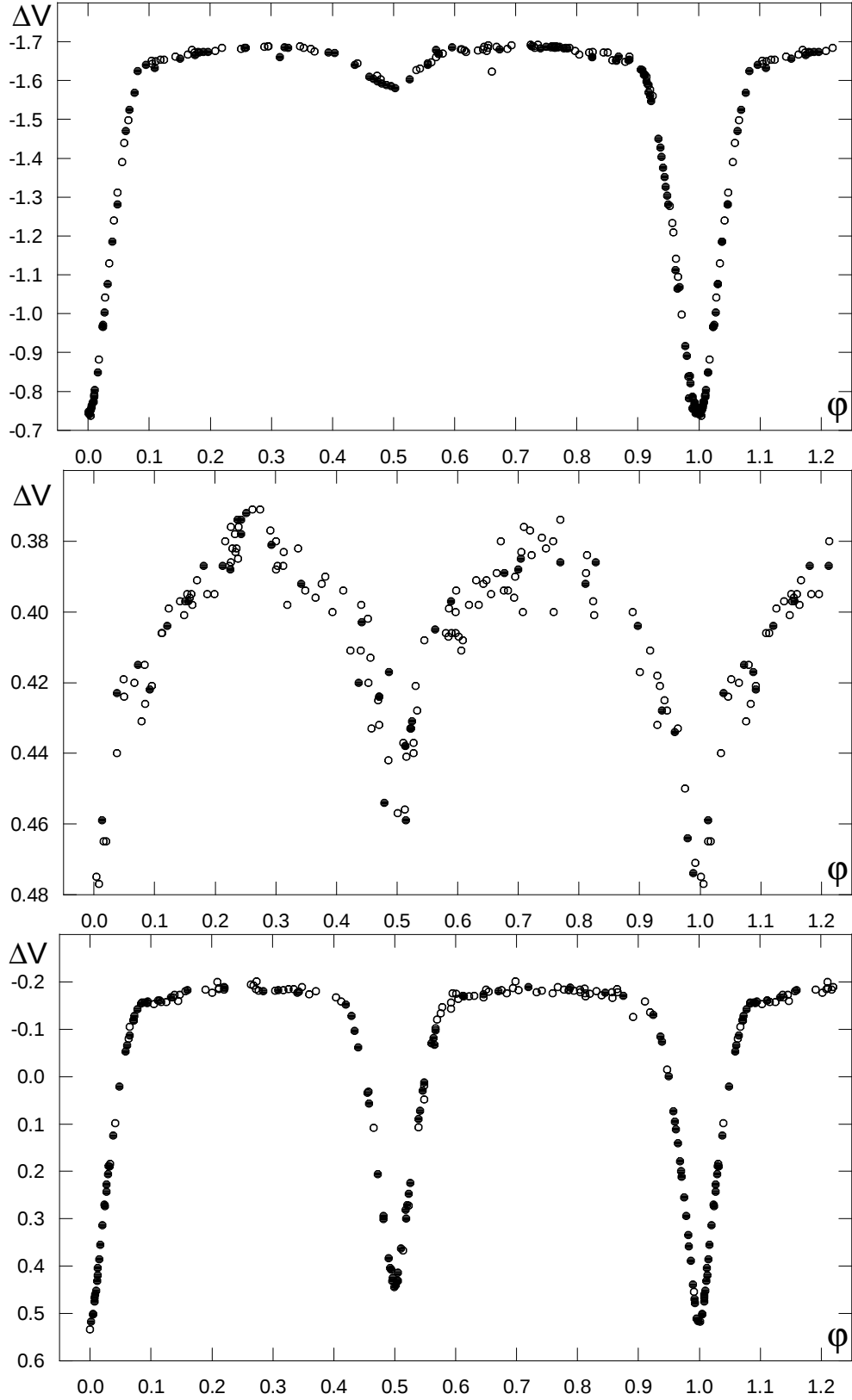
Figure 2: Top to bottom: phase diagrams of \delta Lib, IM Mon and U Oph.
