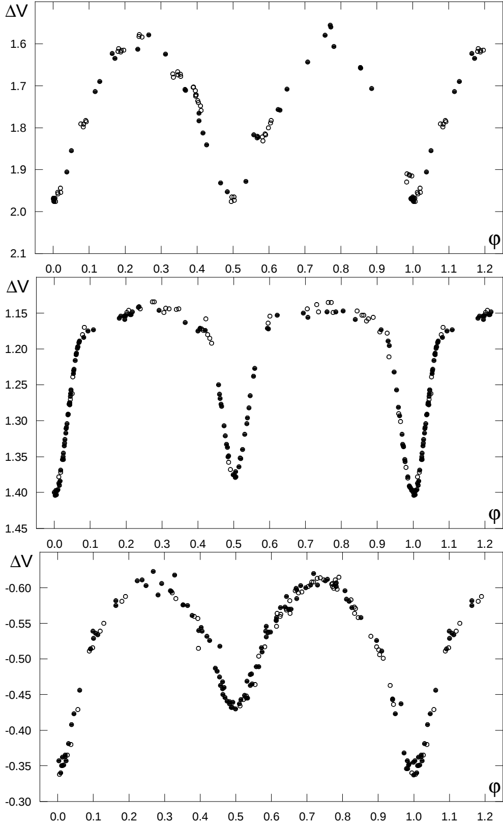
Figure 6: Top to bottom: phase diagrams of V453 Sco, V906 Sco and \mu^1 Sco.
