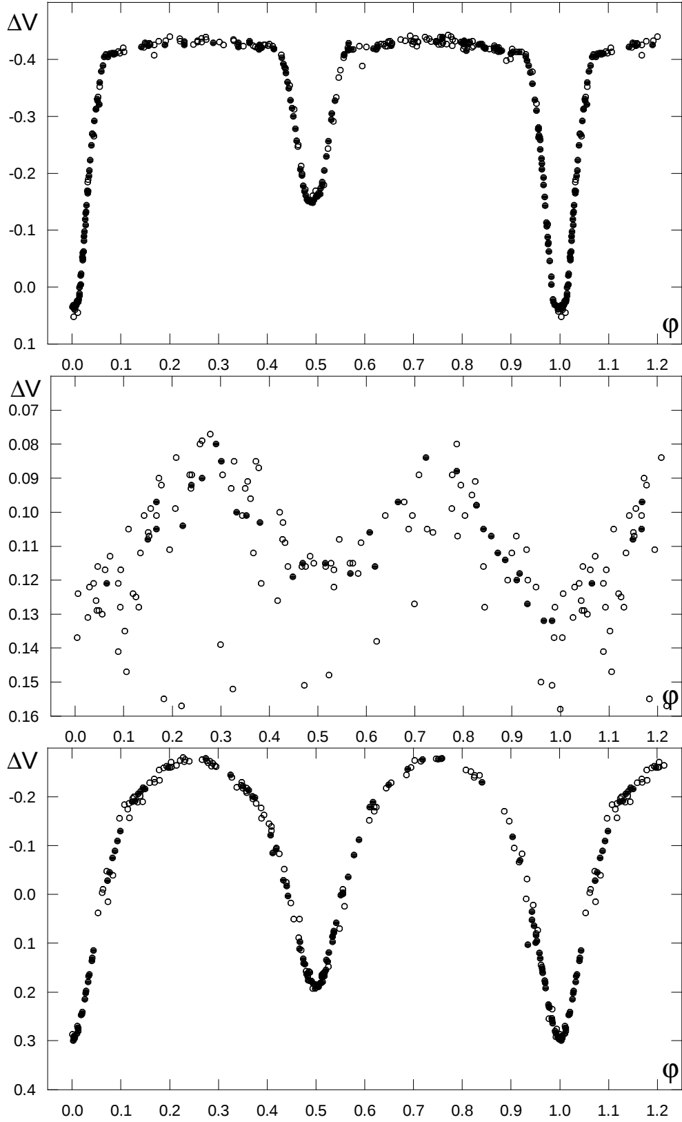
Figure 4: Top to bottom: phase diagrams of \zeta Phe, UU Psc and V Pup.
