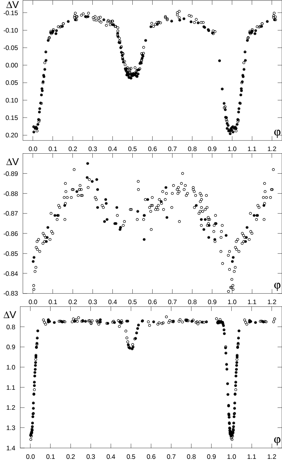
Figure 3: Top to bottom: phase diagrams of VV Ori, \psi Ori and EE Peg.
