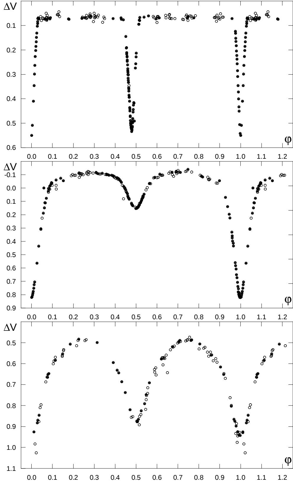
Figure 5: Top to bottom: phase diagrams of VV Pyx, RS Sgr and V3792 Sgr.
